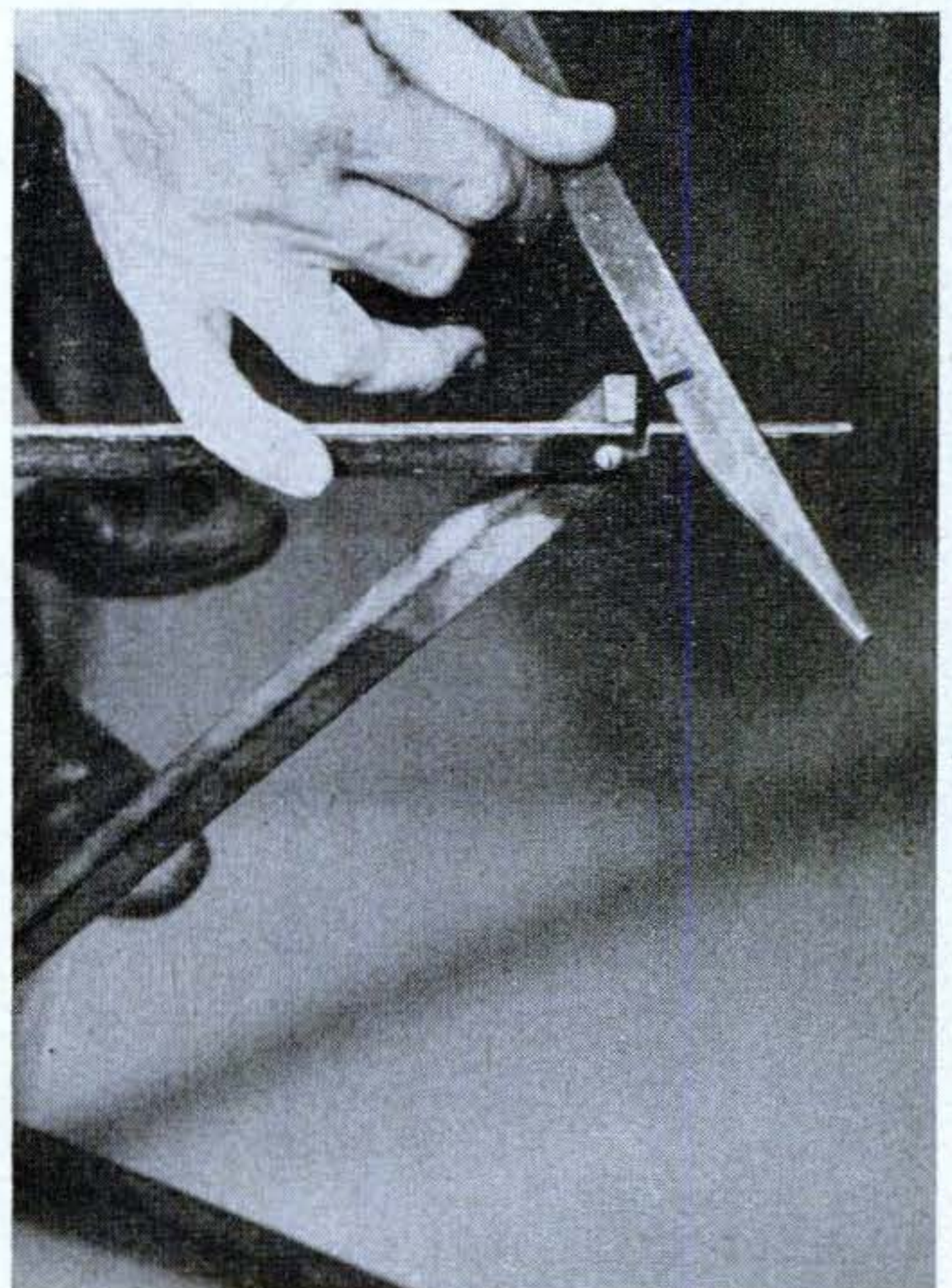
Notch top rails and stretchers accurately to form a flush joint for the glass to rest upon.
